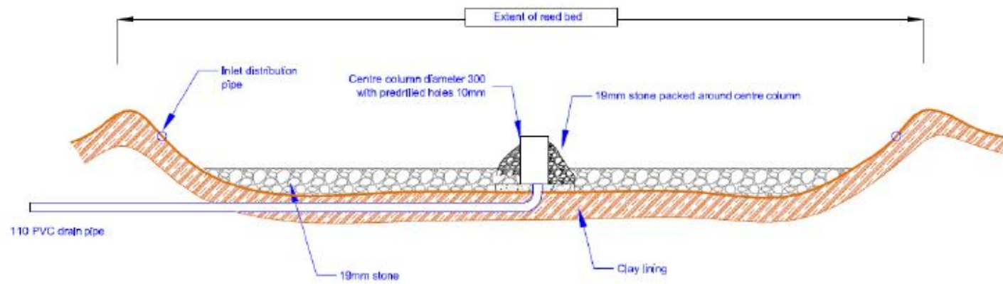
Typical section through a constructed reed bed
