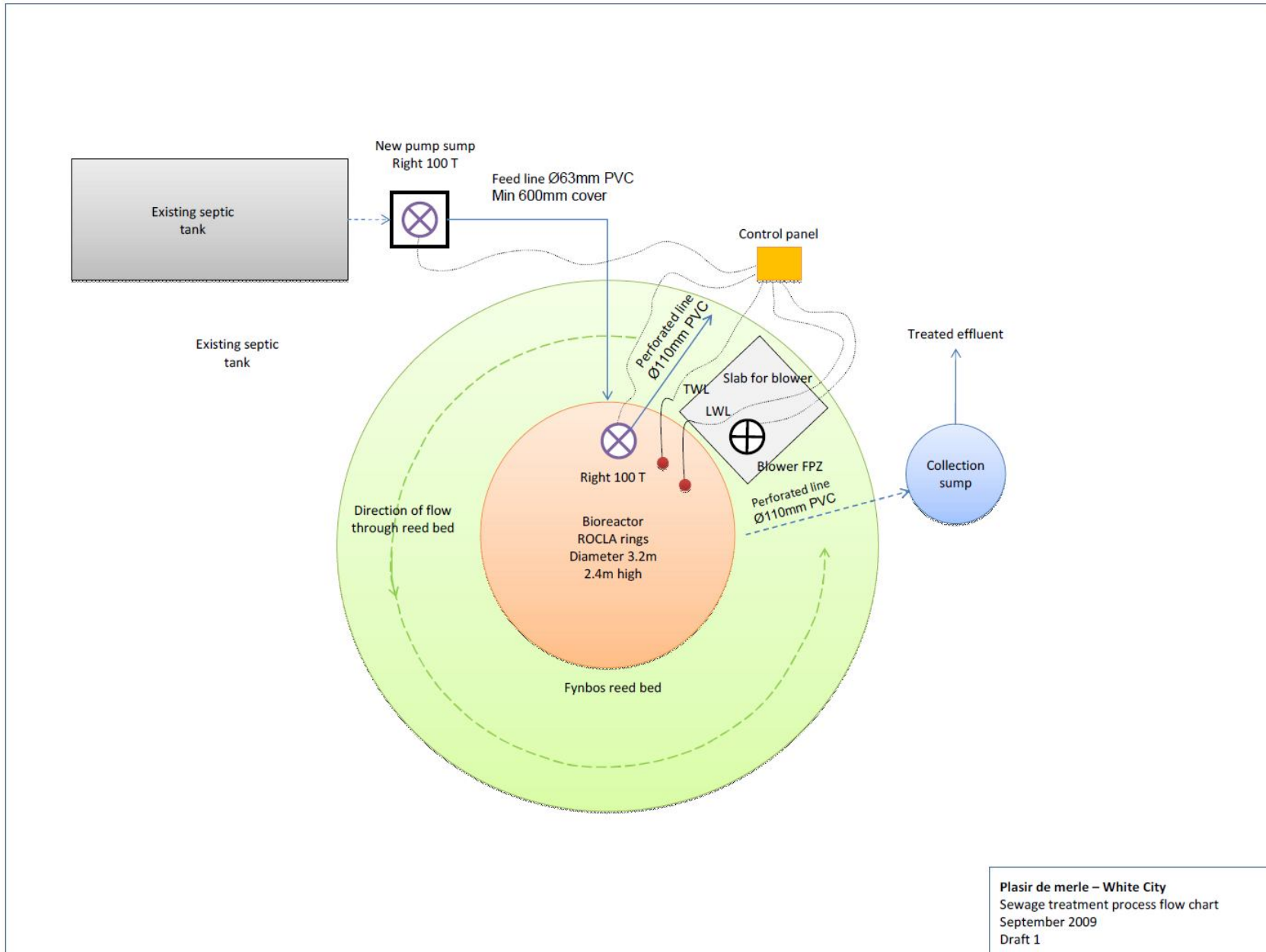
Figure 1: Line diagram/ illustration of the proposed activate sludge biological reactor.
